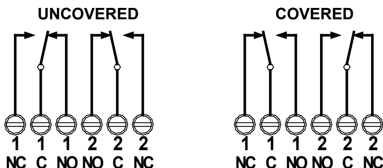
FAIL-SAFE "HIGH" RELAY CONTACT POSITION
